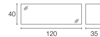
CS/6026-42 CONTENITORE RIBALTA CS/6026-42 DROP-DOWN DOOR UNIT
